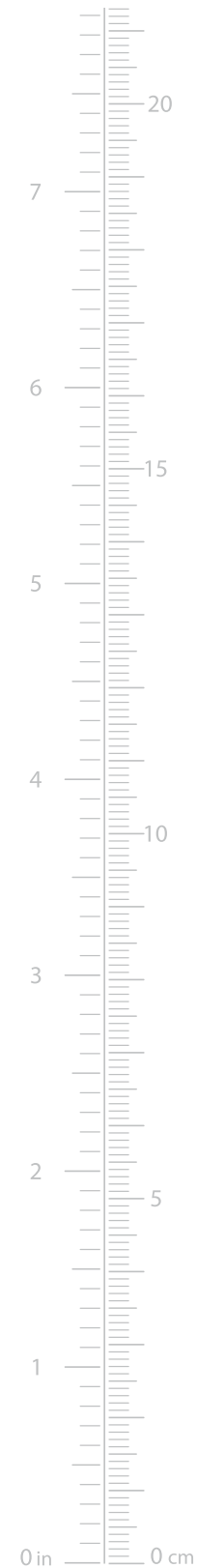
440069 DIAMOND FLÜT ŞAMPANYA CHAMPAGNE FLUTE v:~170 cc. 5 3/4 US oz. 6 UK oz. h: 206 mm. 8" t: 62 mm. 2 1/2" b: 68 mm. 2 3/4" d: 68 mm. 2 3/4" SKU / PACKING 1079544* fk12/fb12
